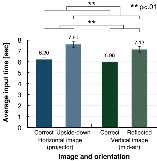
Fig. 14 Results of user study
